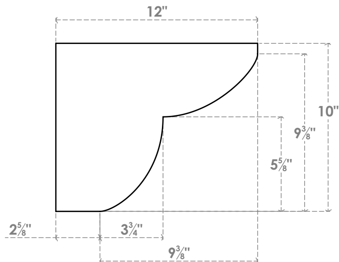
SIDE PROFILE
