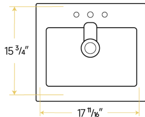
Cutout Size
