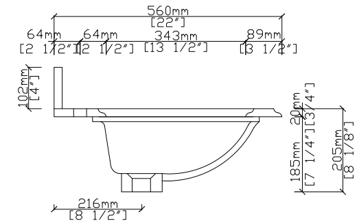
RIGHT VIEW
