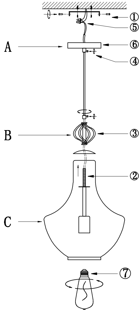
Installation sequence diagram
