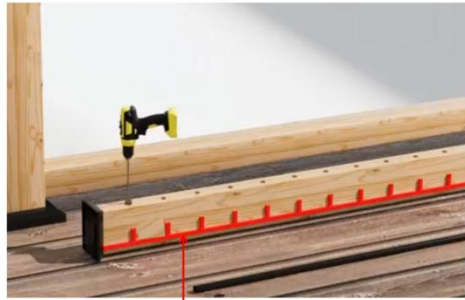
Center spacing is 4.5 inches
