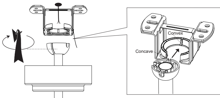
Safety rope installation method
