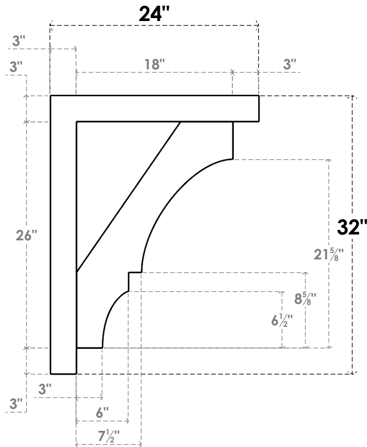
SIDE PROFILE
