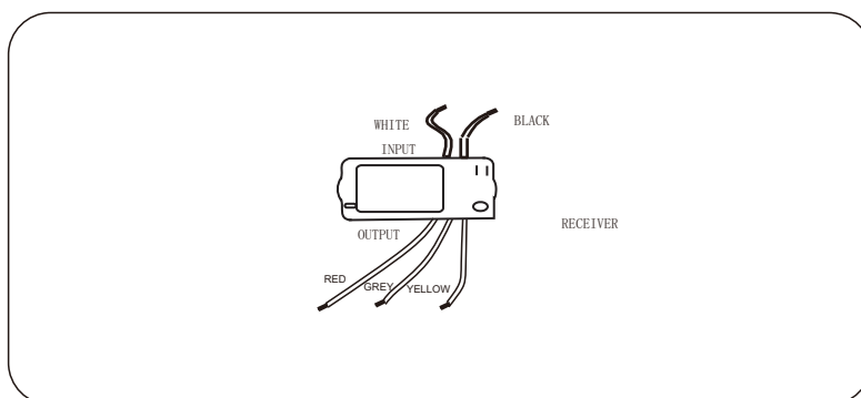
For Mounting Controller,Model T101B
