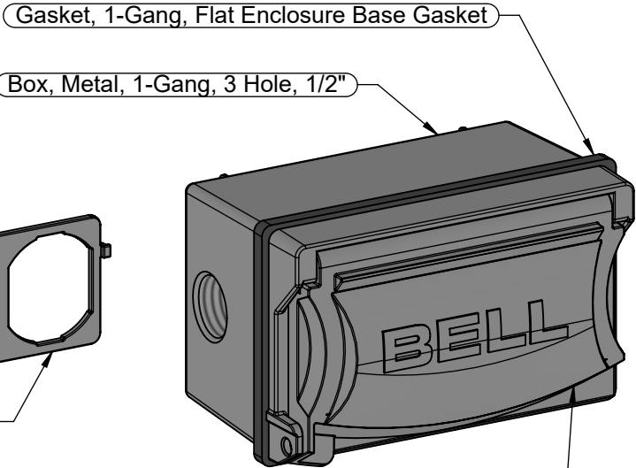
COVER, FLAT, METAL, 1-GANG, HORIZONTAL
