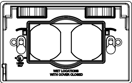
SHOWN WITHOUT COVER SCALE 1:2
