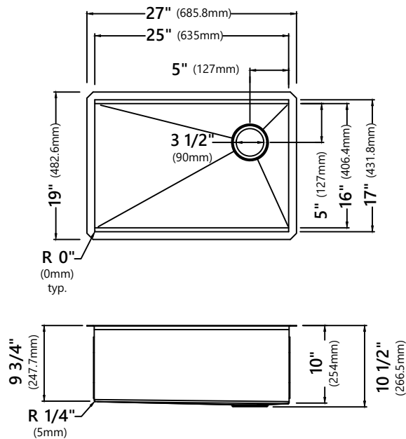
Model #: KWU110-27/PGM Sink Dimensions: 27" x 19" x 10" Min Cabinet Size: 30"
