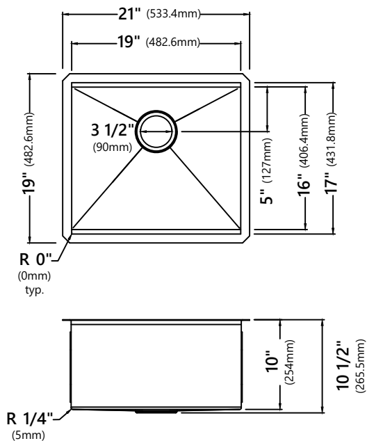
Model #: KWU111-21 Sink Dimensions: 21" x 19" x 10" Min Cabinet Size: 24"
