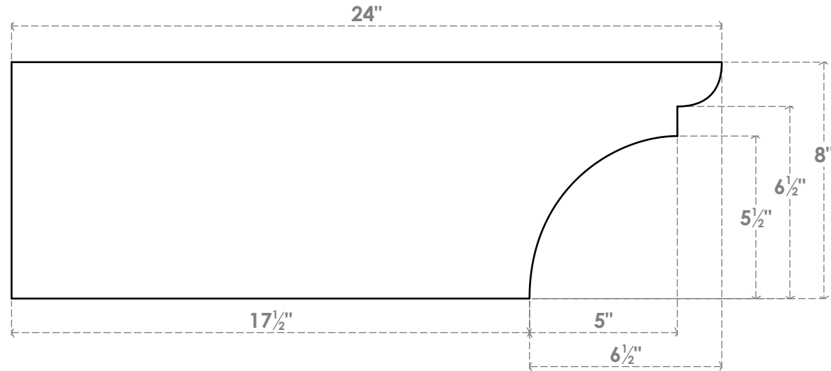
SIDE PROFILE
