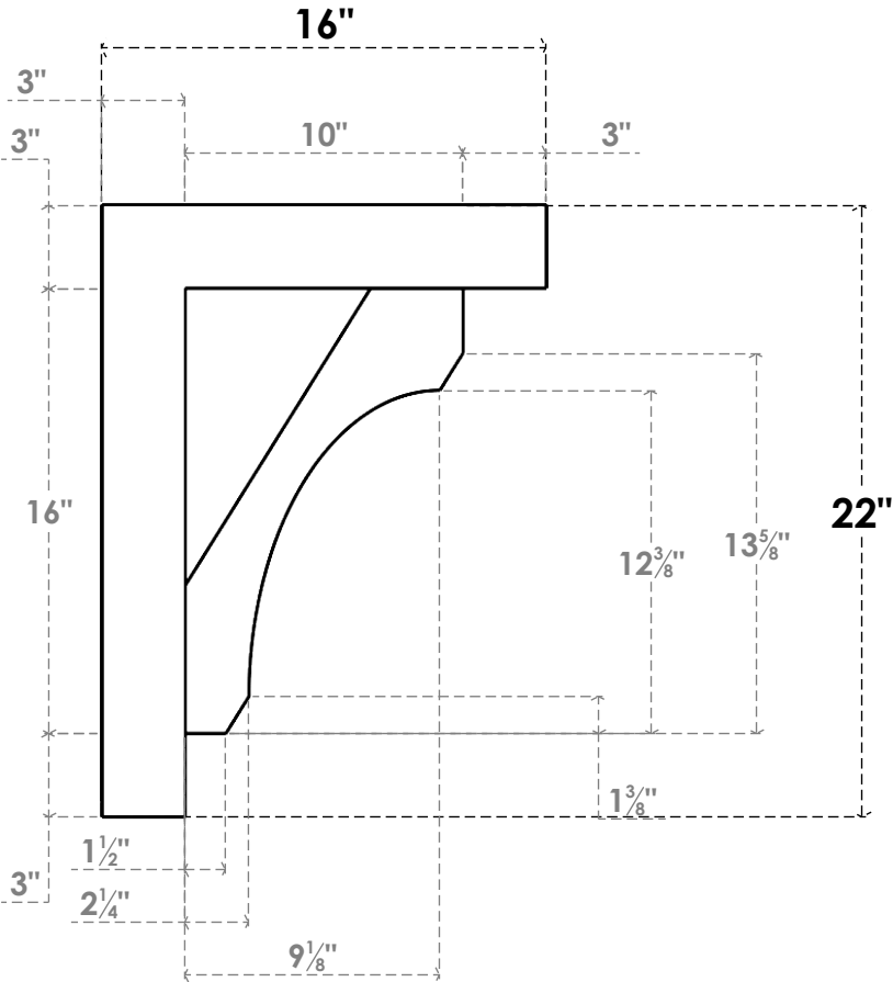
SIDE PROFILE
