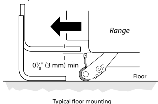
Fig. 12.25 Anti-Tip bracket
