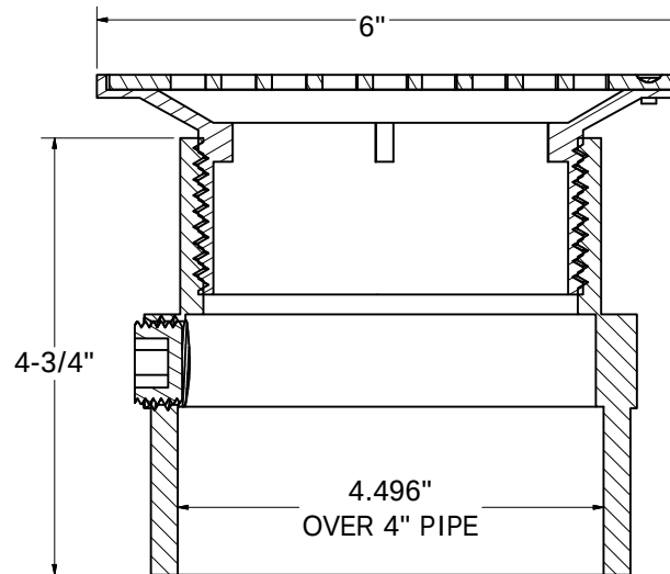
SECTION A-A SCALE .9
