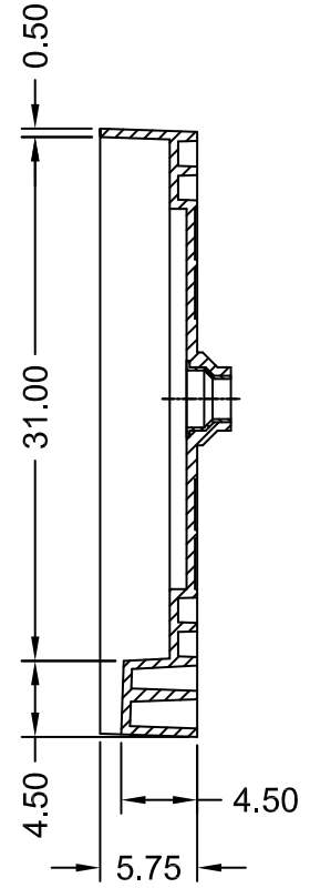
SECTION B-B
