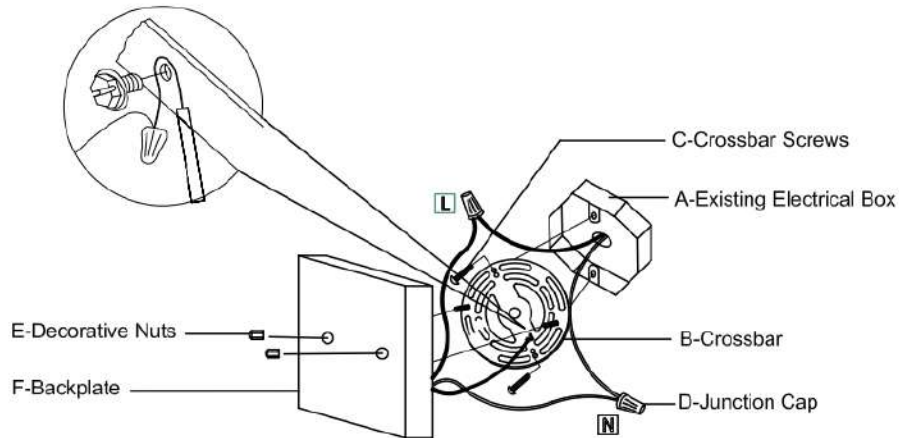
Wire Connection Diagram:
