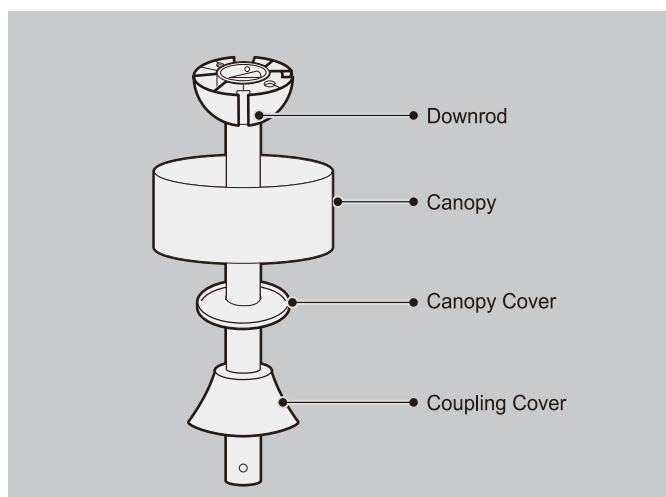
② Assemble the canopy, canopy cover and coupling cover to the downrod in turn.
