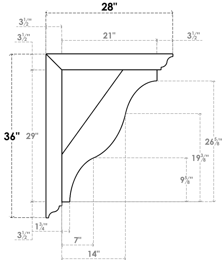
SIDE PROFILE
