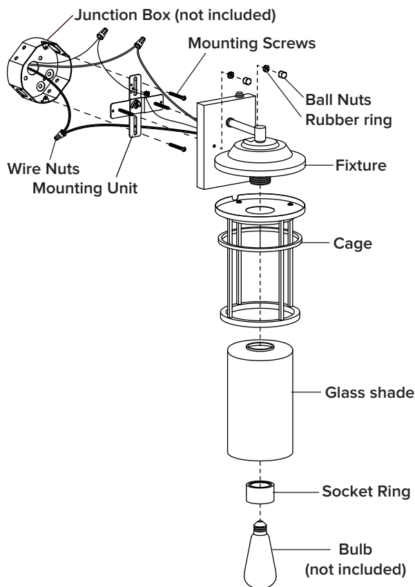
Fixture
