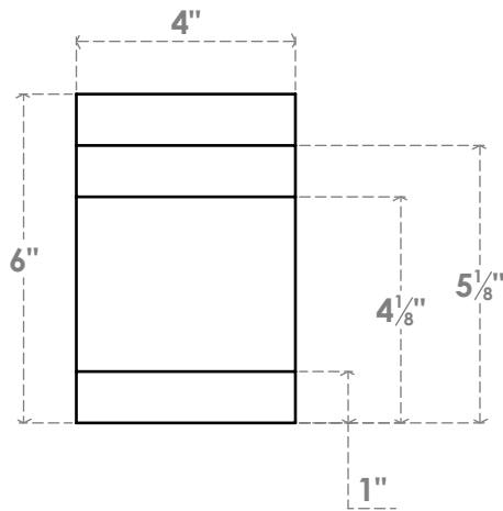
FRONT PROFILE
