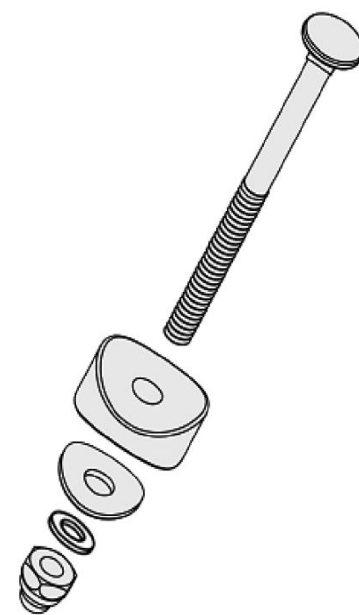
11 Screw(of safety pole)/12pcs
