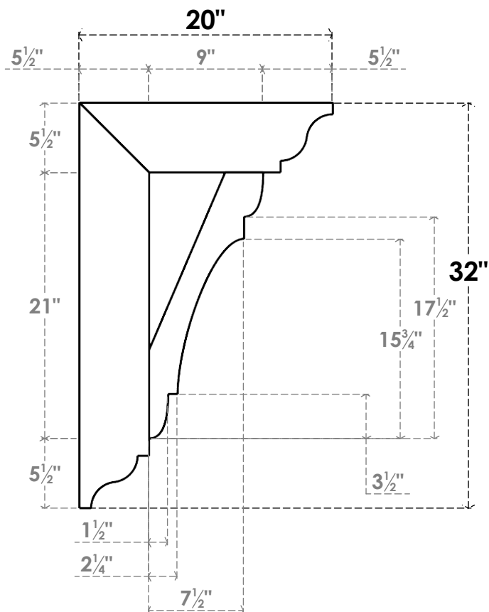
SIDE PROFILE
