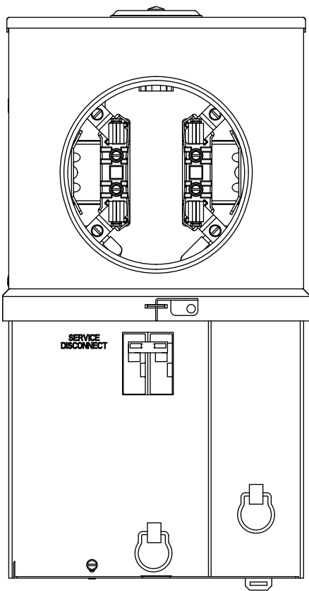
View Shown with Lower Cover Removed
