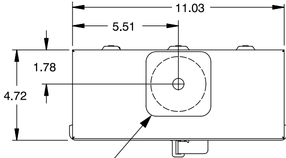
TYPE RX (SMALL) HUB PROVISION CLOSURE PLATE INSTALLED
