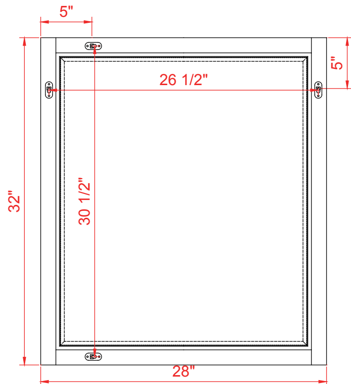
BACK VIEW
