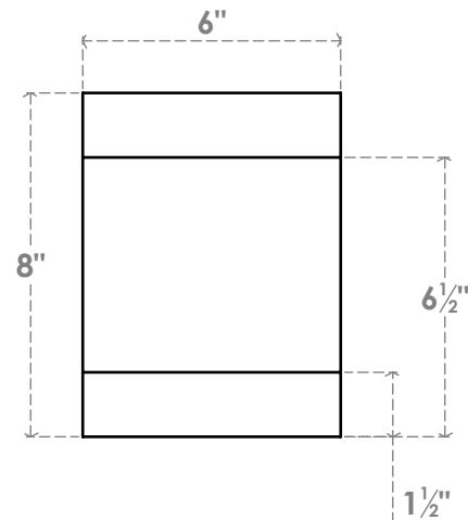
FRONT PROFILE
