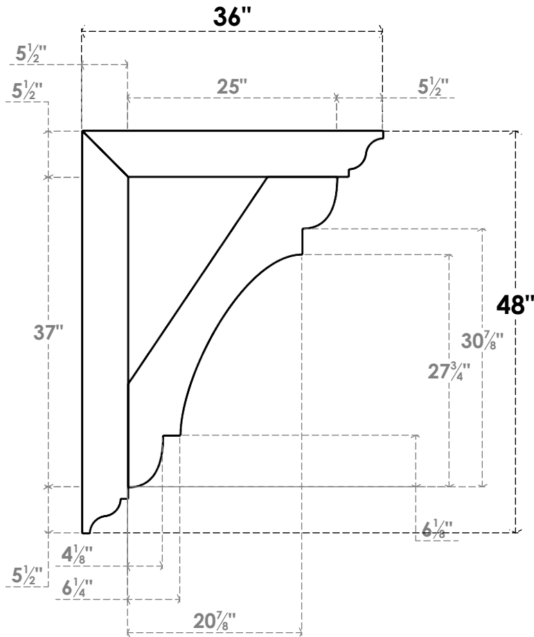
SIDE PROFILE
