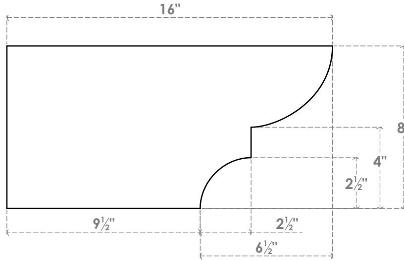
SIDE PROFILE
