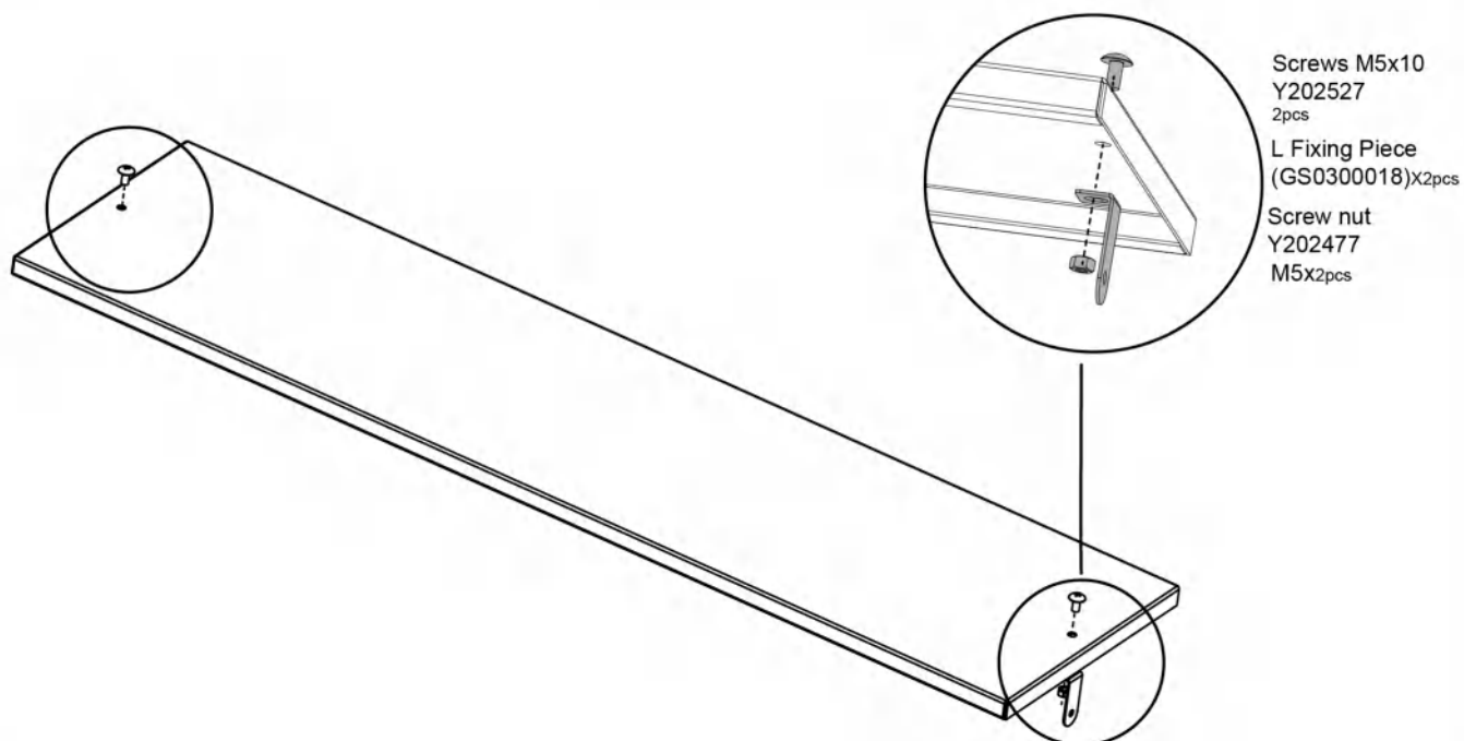
Shelf (GS0300009)X2pcs
