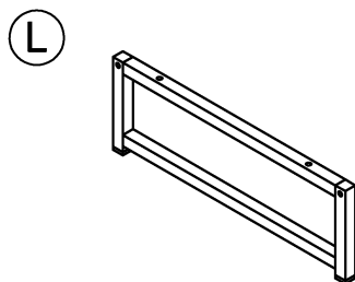
SIDE METAL FRAME 17.68" X 5.9" X 0.75" 2PCS
