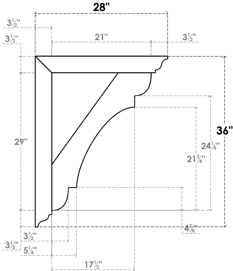
SIDE PROFILE
