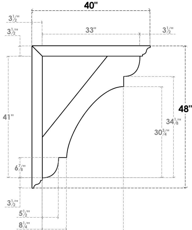
SIDE PROFILE
