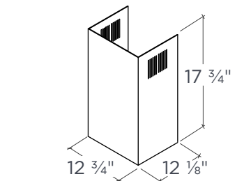
UPPER CHIMNEY COVER
