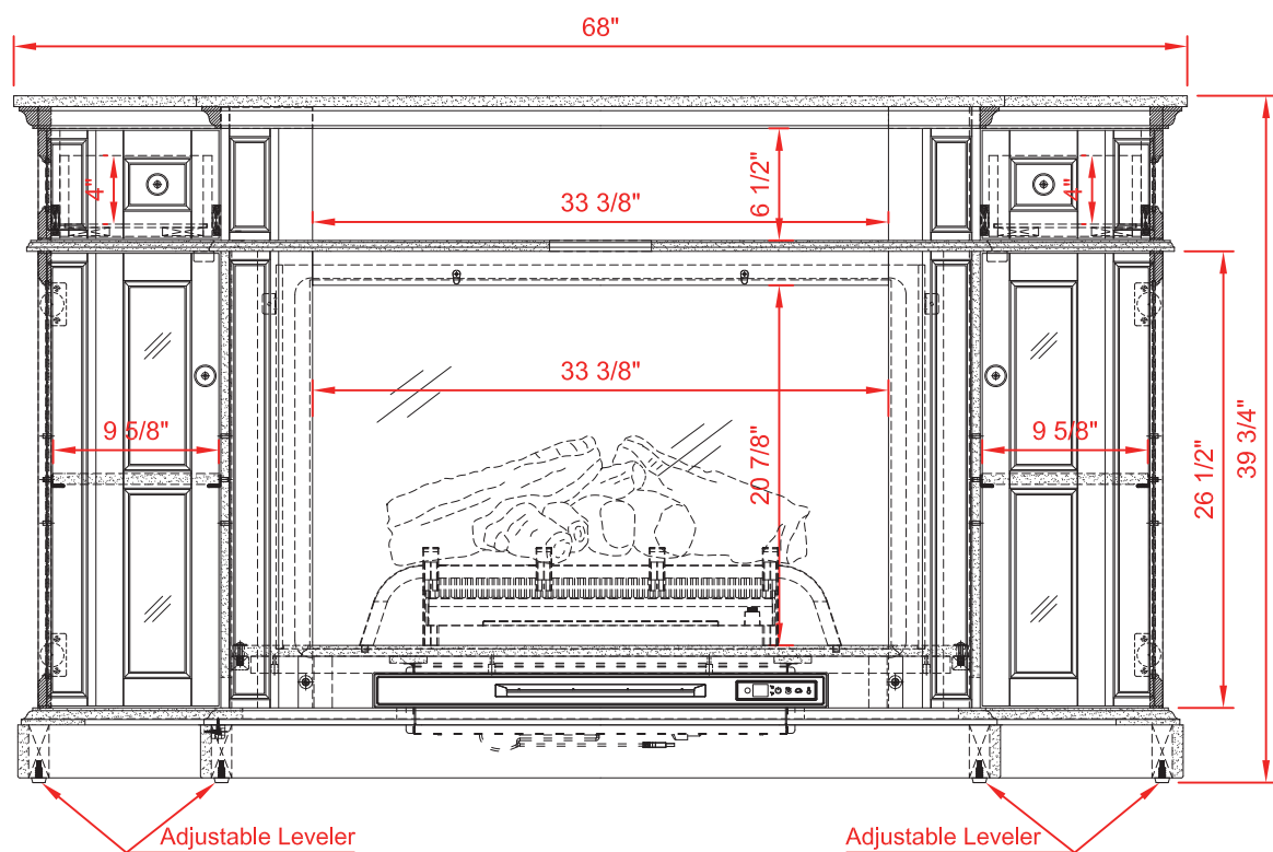
FRONT VIEW
