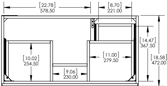
Top View / Vista Superior
