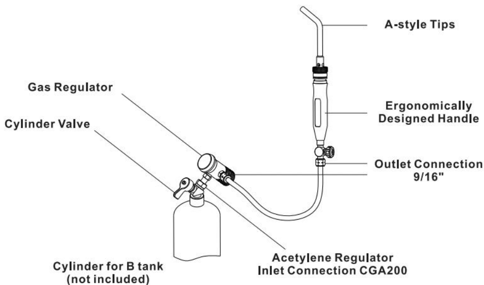
Torch setup
