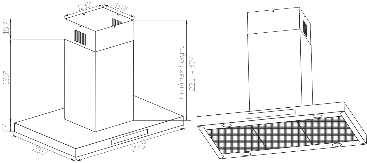
FRONT VIEW
