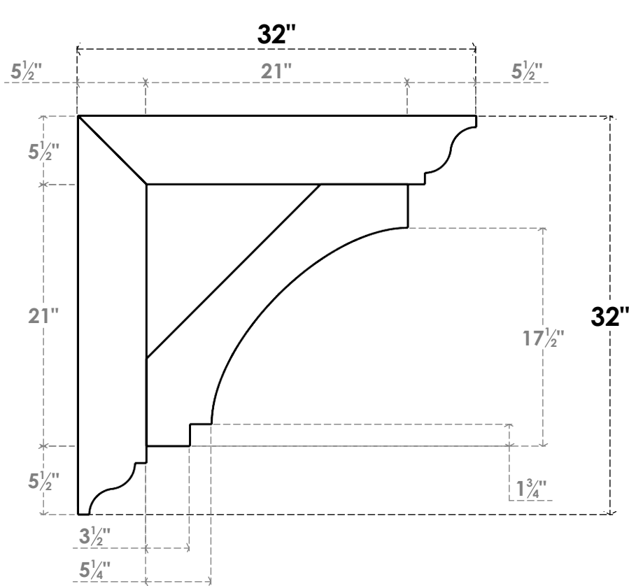
SIDE PROFILE
