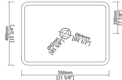
SINK VIEW
