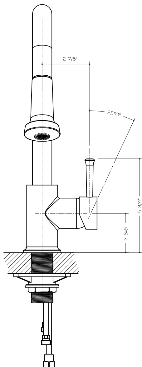
FRONT VIEW
