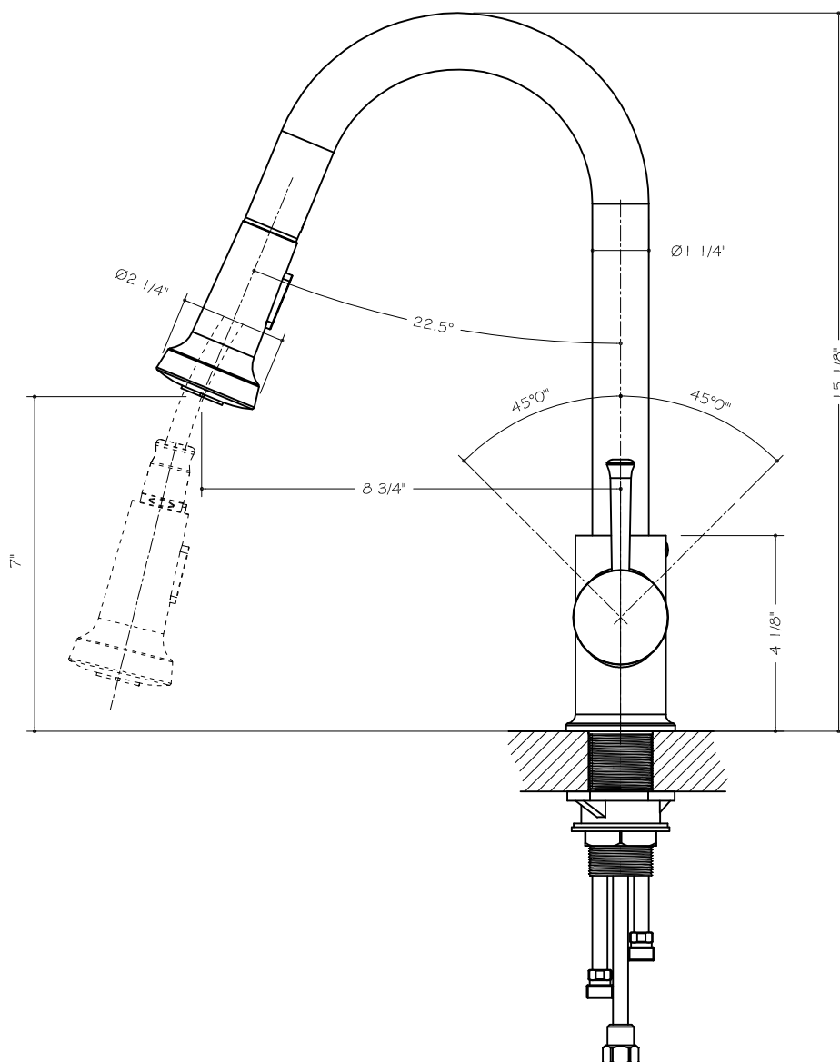
SIDE VIEW
