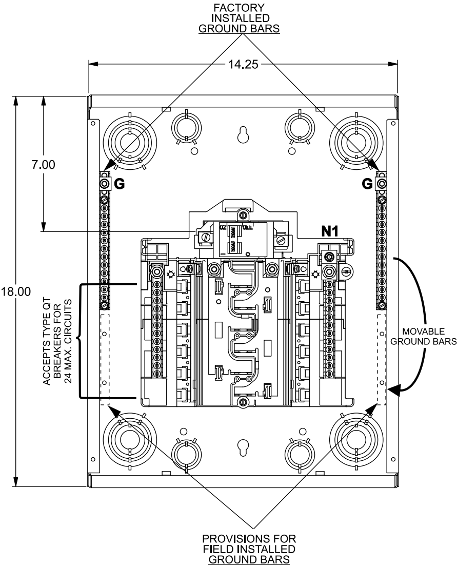
VIEW SHOWN WITH TRIM ASSEMBLY REMOVED
