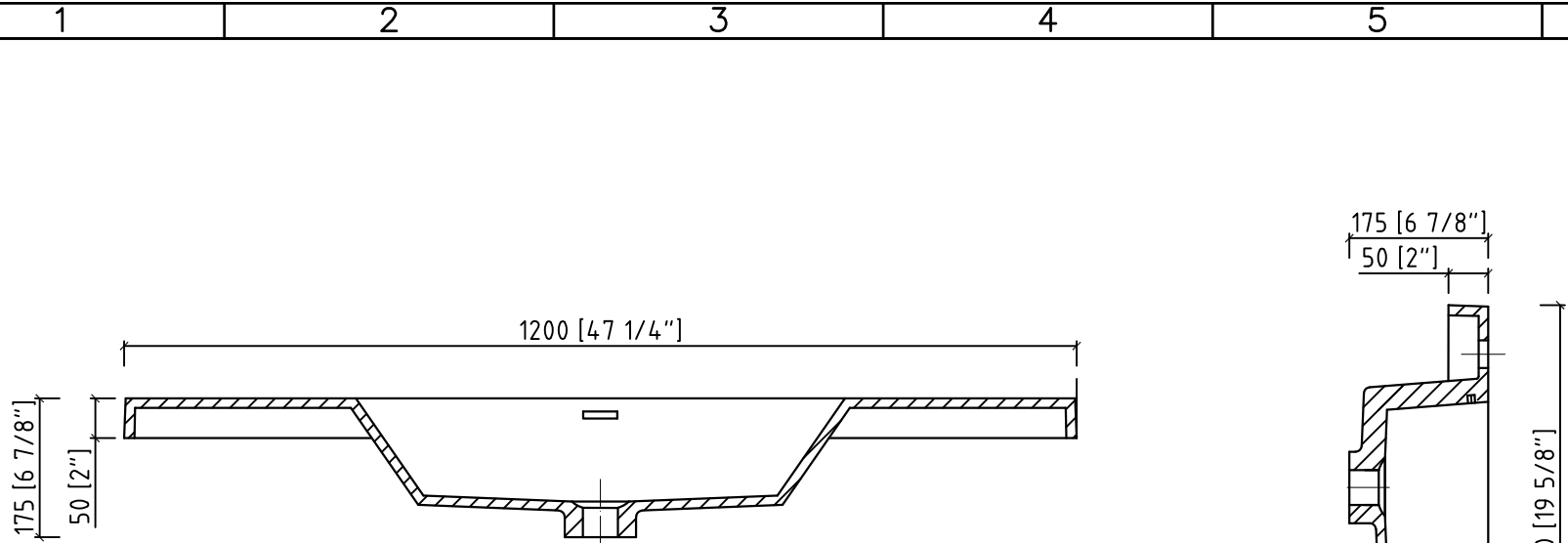
SECTION B-B
