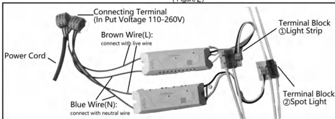
(Figure 3: Plug and Driver)
