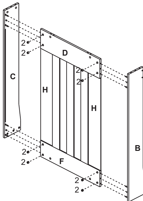
Cam Lock Fastening System
