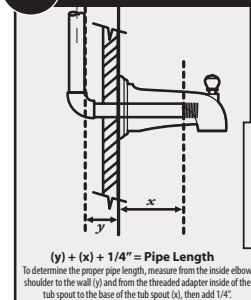
4.3A Tub Spout Installation
