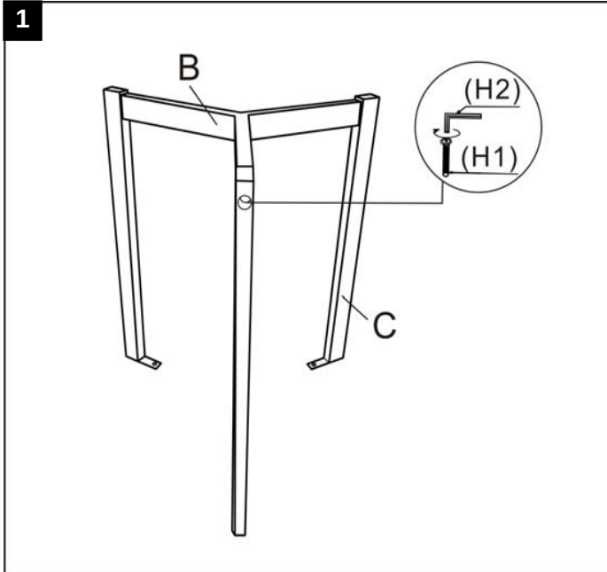
Step 1 Attach legs ( C ) to base ( B ), using allen bolt L ( H1 ) Tighten with allen key ( H4 )
