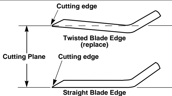
End view of blades, comparing twisted and straightened blades
