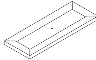
8 Drawer Front Qty 1 (13.66×5.11×0.59")
