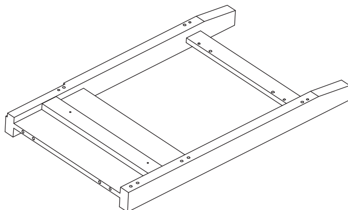
2 Side Panel (Left) Qty 1 (14.88×25×1.96")
