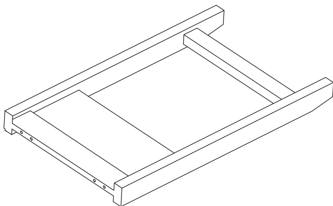
3 Side Panel (Right) Qty 1 (14.88×25×1.96")
