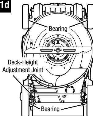
For LM2020/LM2020-FC
