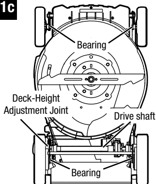
For LM2020SP/LM2020SP-FC
