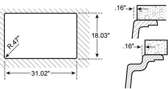
TRIN100XLDM Undermount Cut-out
