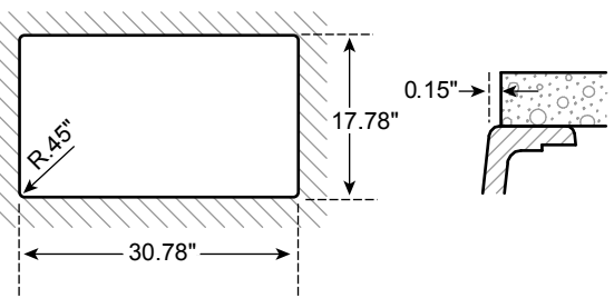
SIGN100XLDM/SIGN200DM Undermount Cut-out
