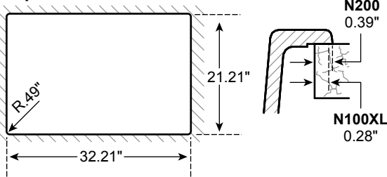
SIGN100XLDM/SIGN200DM Undermount Cut-out
