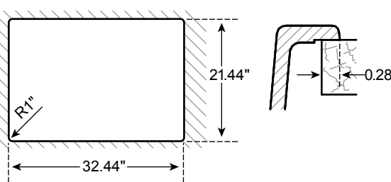
TRIN100XLDM Topmount Cut-out
