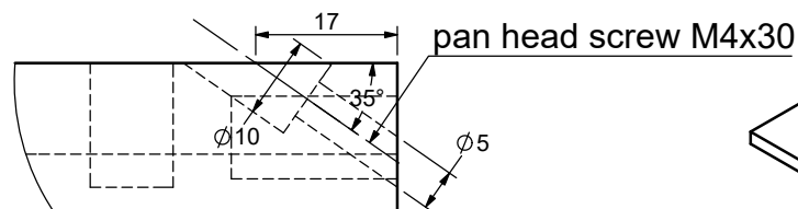
DETAIL AM SCALE 1 : 1
