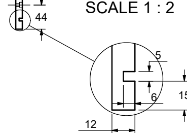
DETAIL AS SCALE 1 : 2
