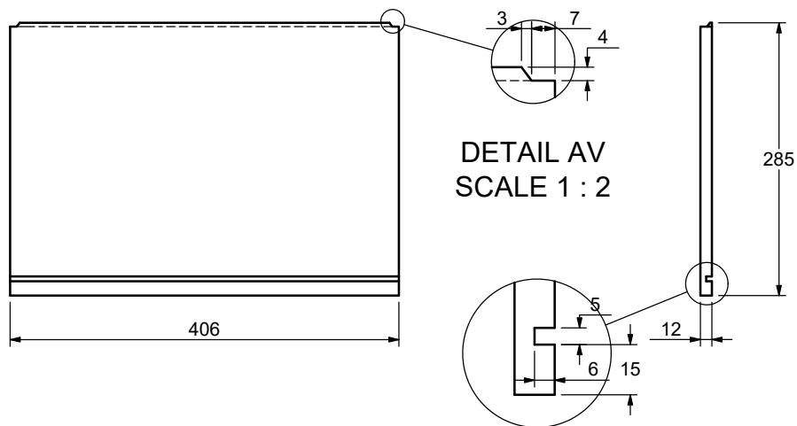
Lower drawer side
