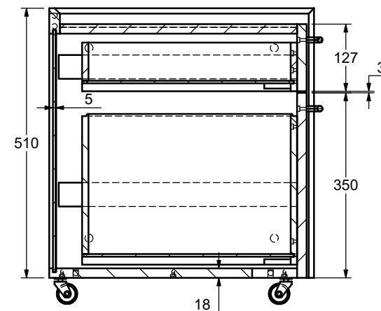
SECTION AD-AD
