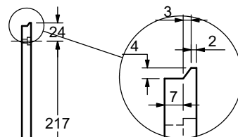
DETAIL AT SCALE 1 : 2
